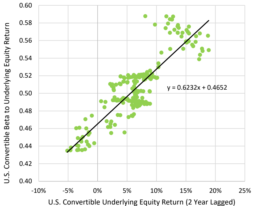
Figure 3. Regression of U.S. 10 Year Convertible Beta to Underlying Equity Return vs. U.S. 10 Year Convertible Underlying Equity Return (2 Year Lagged) 6
